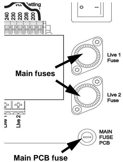
Figure 25: Fuses
