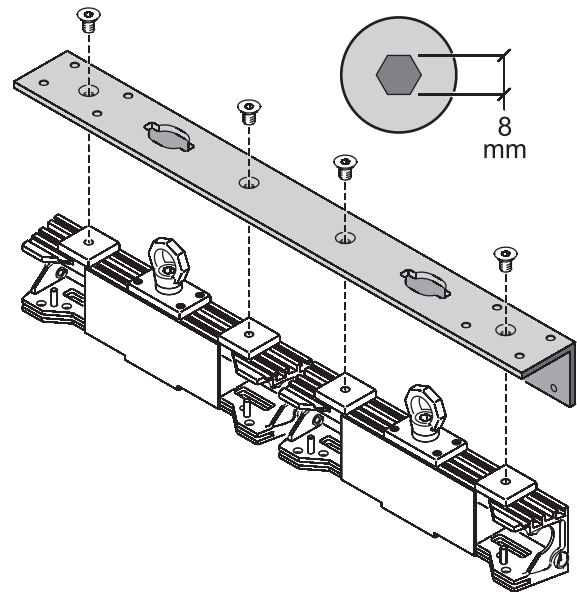
Figure 5: Header Connection Bracket (Double Header illustrated)
