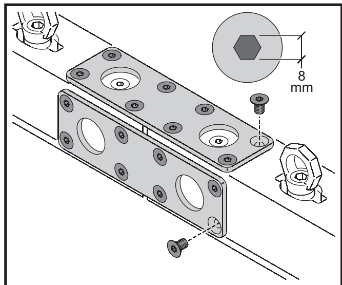
Figure 6: Joining Plates for Header Connection Brackets
