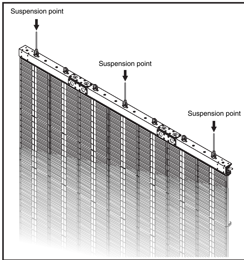
Figure 7: Installation 7 panels wide
