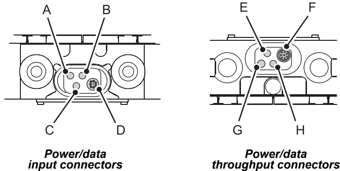
Figure 9: Power and data connectors
