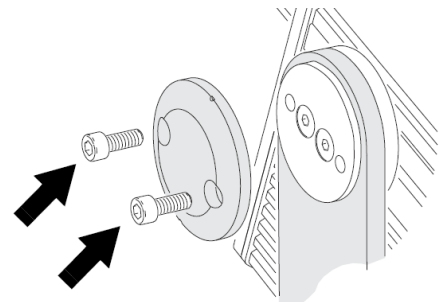
Figure 2. Tilt adjustment
