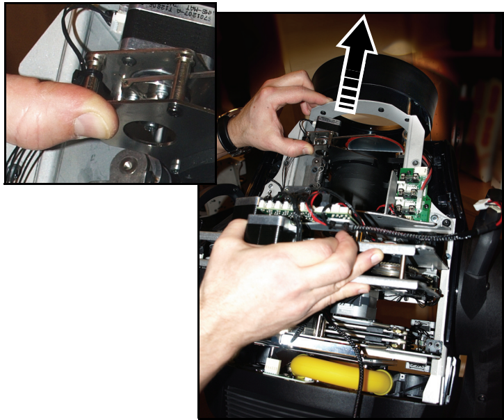
Figure 17: Removing the projection module
