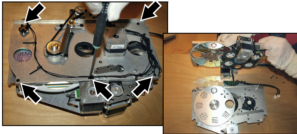
Figure 18: Opening the projection module
