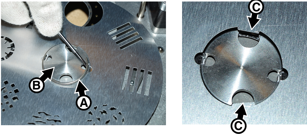
Figure 26: FX wheel removal and mounting
