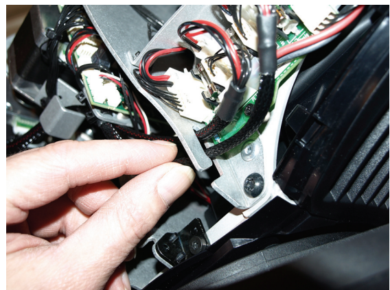
Figure 16: Releasing the projection module connectors
