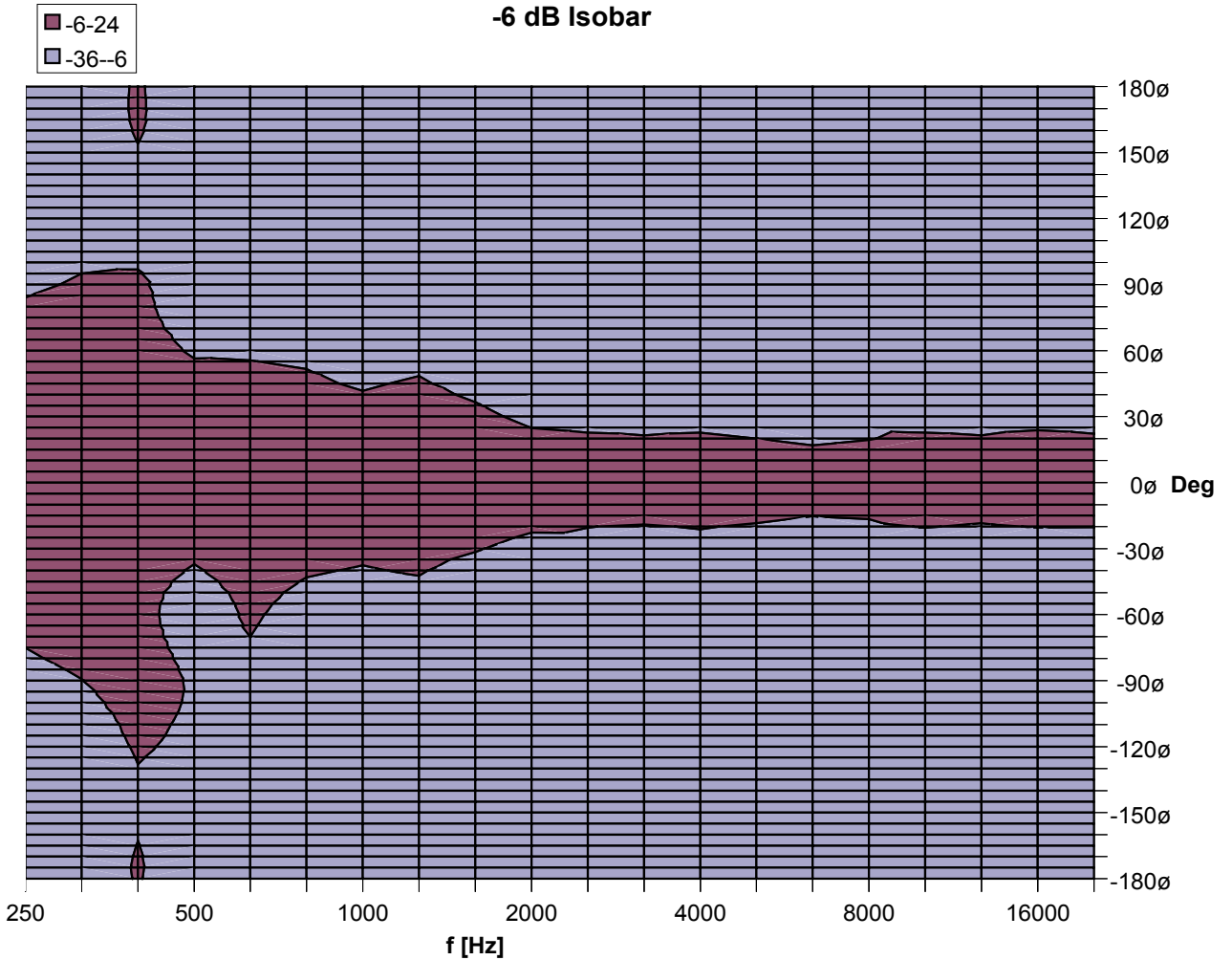
-6 dB Isohar Horizontal
