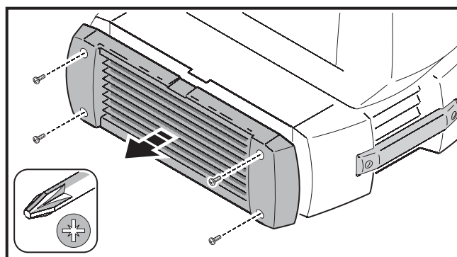
Figure 15: Removing base cover and dimmer unit
