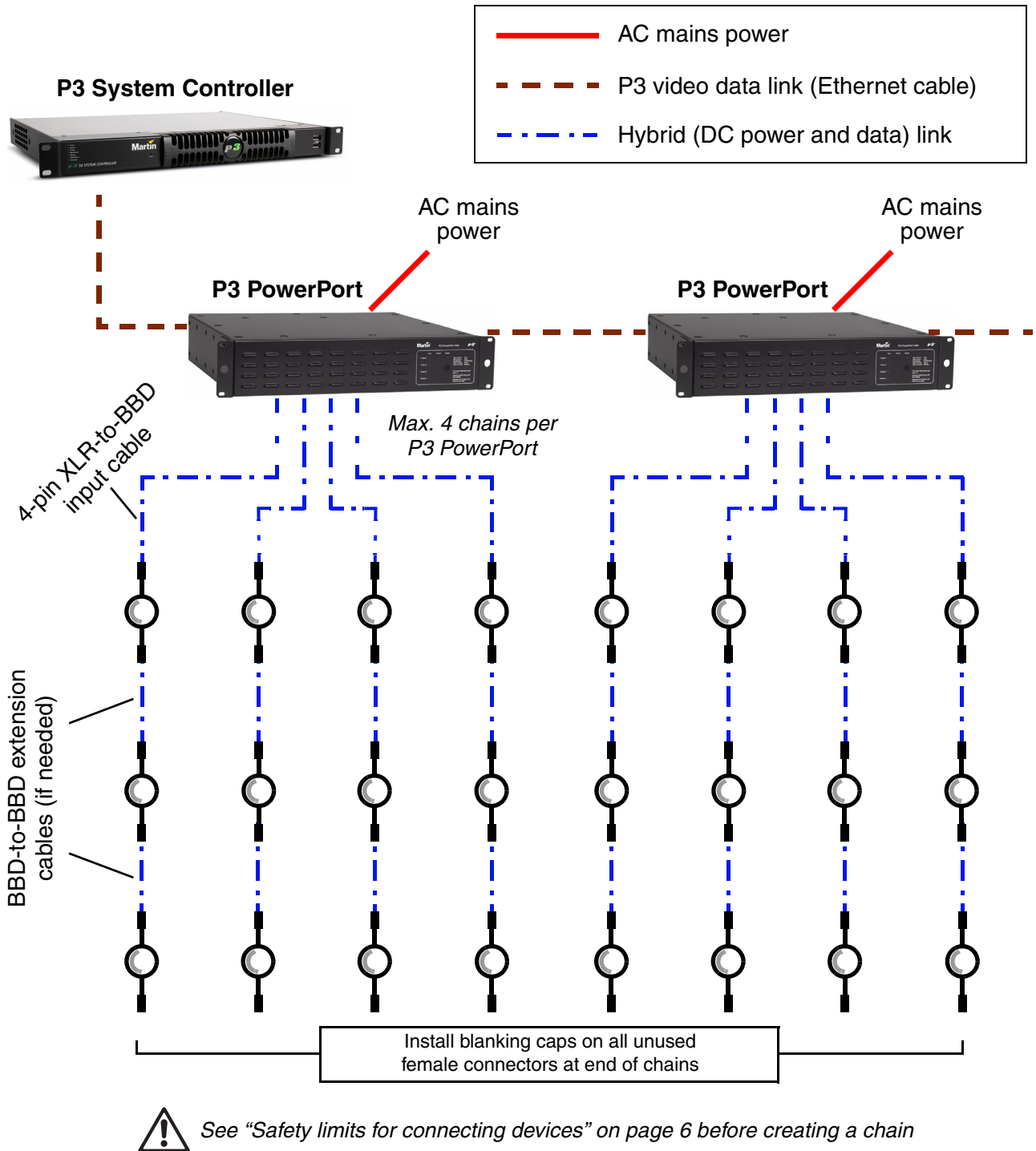
Figure 9: P3 system layout
