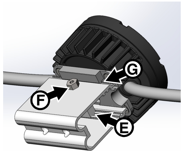
Figure 7: Installing a Dot on a mounting profile
