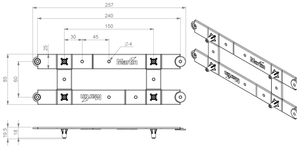
VC-Grid 15/30/60™ Mounting Frame
