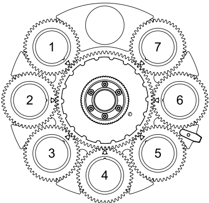
Gobo Wheel 1 (seen from LED side)
