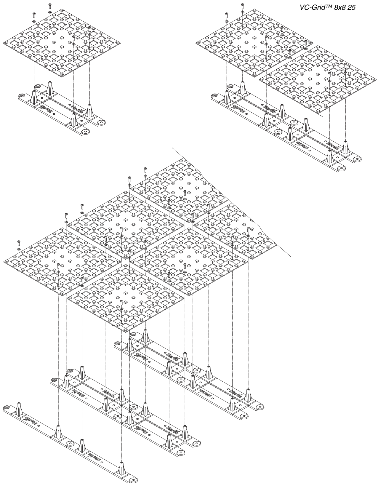
Figure 4. Fastening the VC-Grid to Mounting Frames
