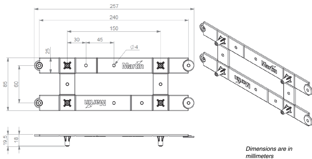
Figure 2. VC-Grid 15/30/60 Mounting Frame dimensions
