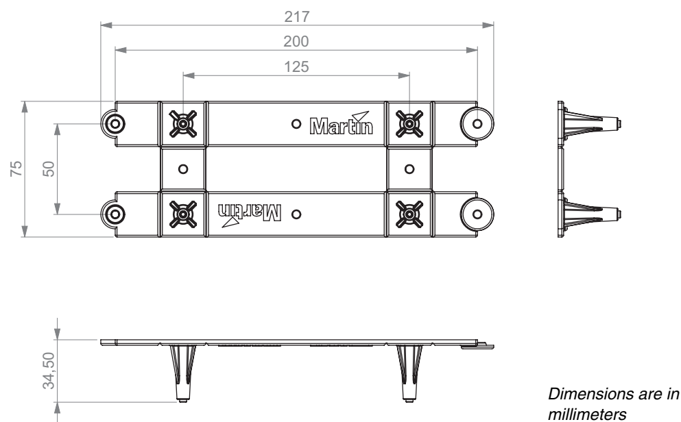
Figure 1. VC-Grid/VC-Strip 25 Mounting Frame dimensions
