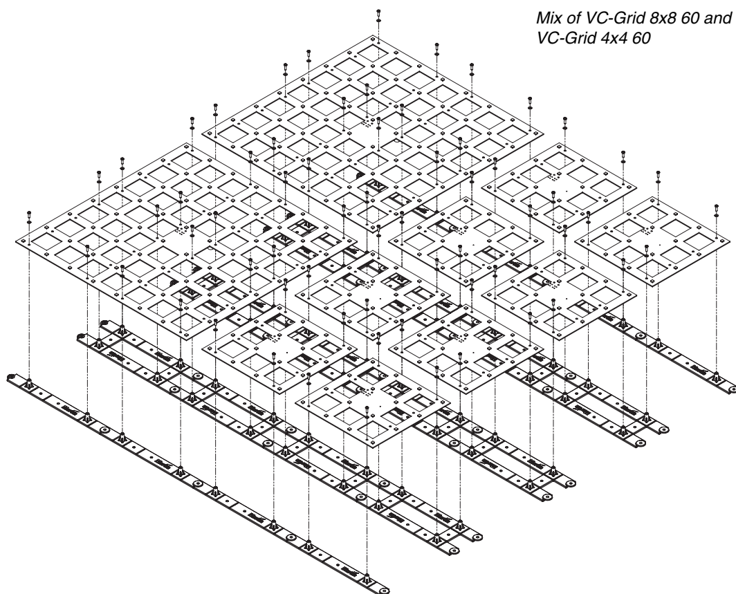
Figure 5. Fastening the VC-Grid to Mounting Frames (contd.)
