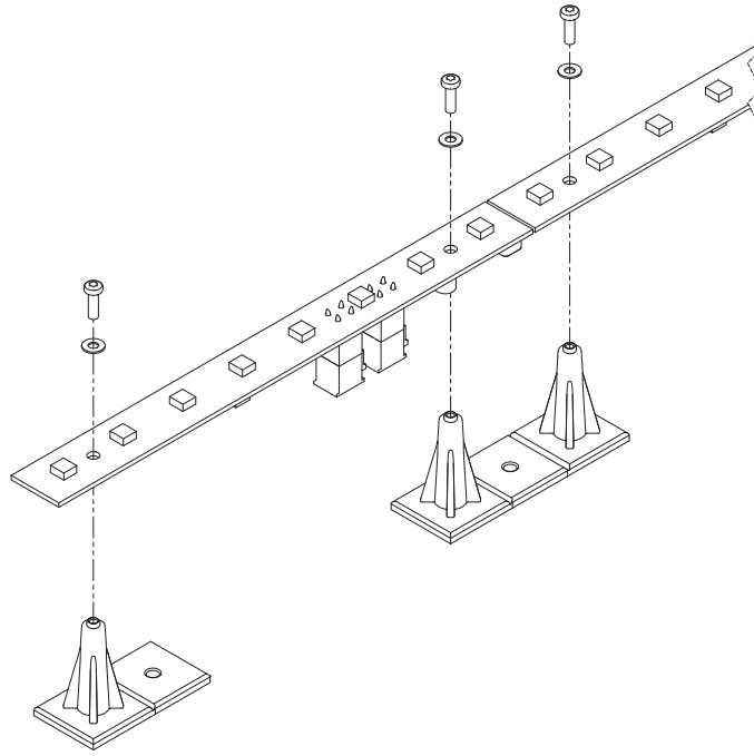
Figure 6. Fastening VC-Strips to Mounting Frame elements
